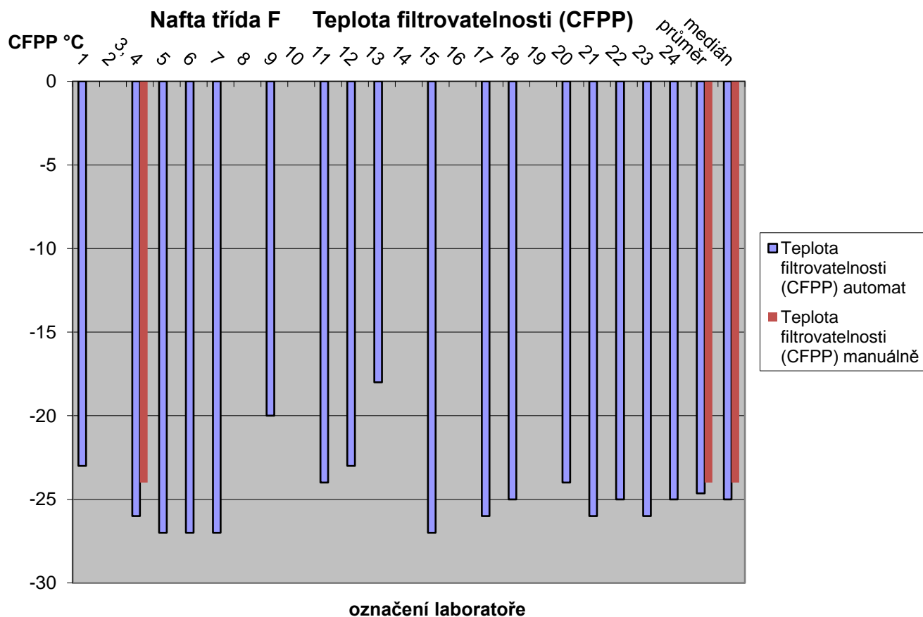
Obr. 14 CFPP
