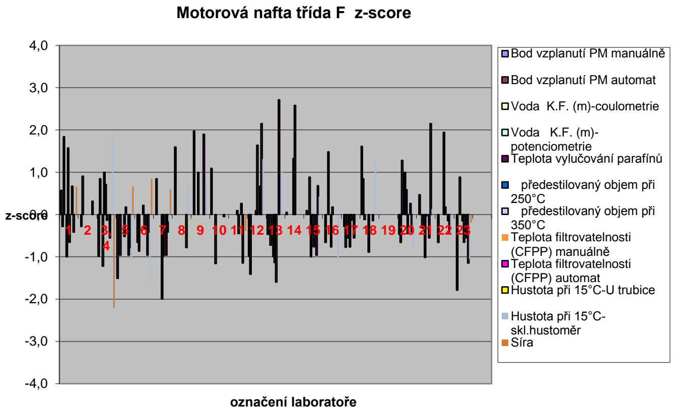
Obr. 18 z – score
